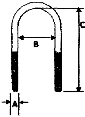
Round Bend
